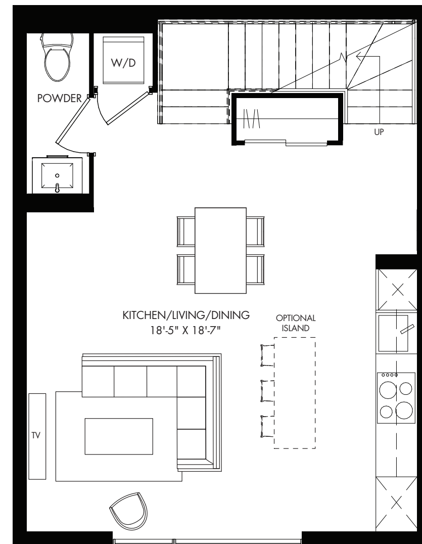
MAIN LEVEL
